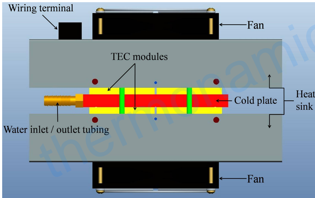
Over-all Structure of the Thermoelectric Cooling units
